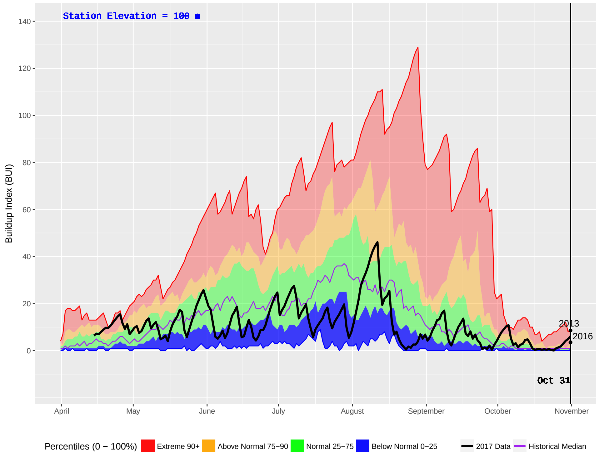
HONNA (93) : Historical (1986–2016) and Current (2017) Noon Buildup Index (BUI)
