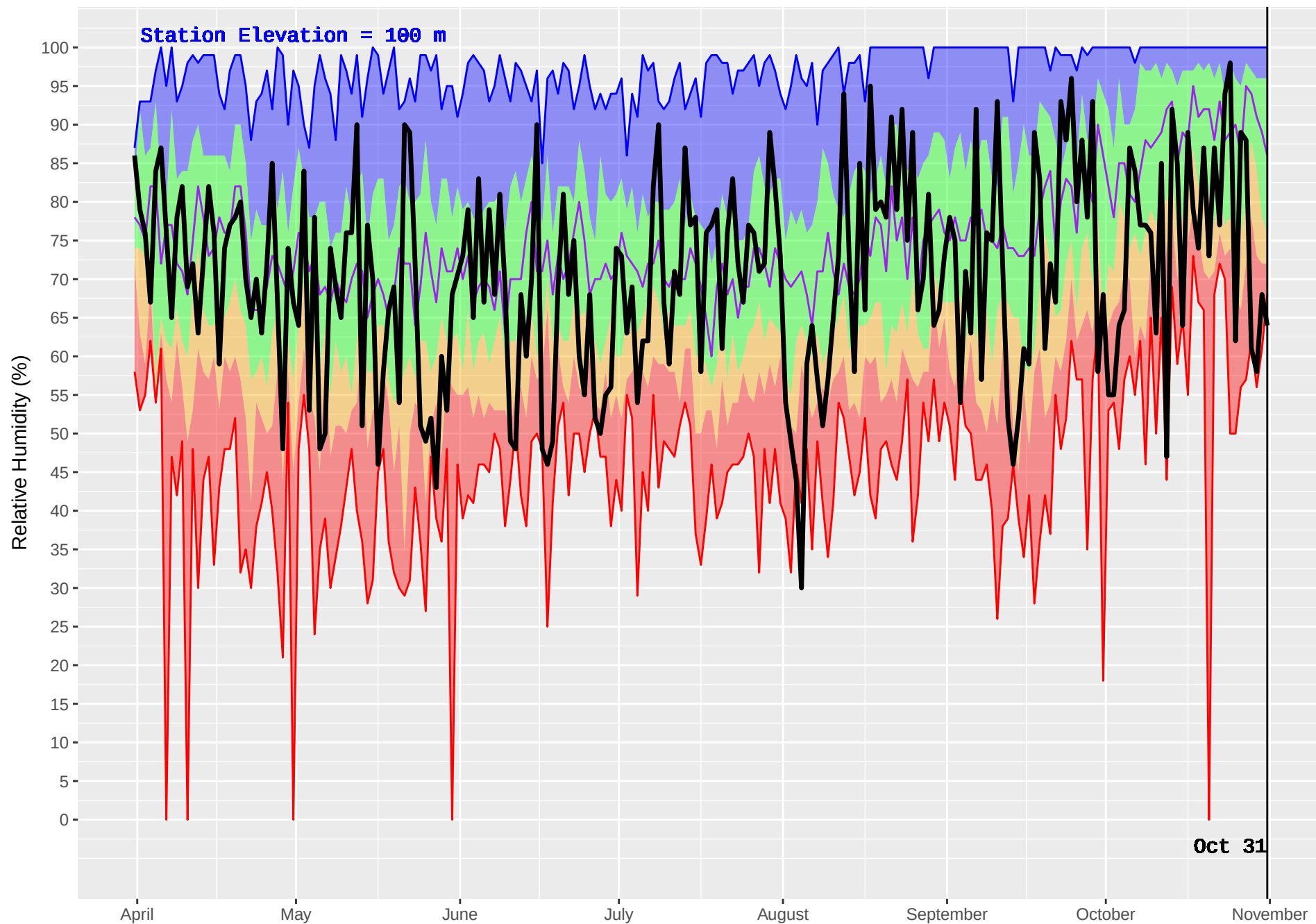
HONNA (93) : Historical (1986–2016) and Current (2017) Noon Relative Humidity
