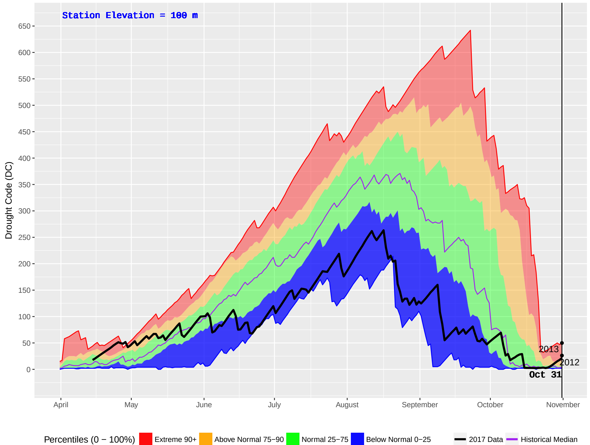
HONNA (93) : Historical (1986–2016) and Current (2017) Noon Drought Code (DC)
