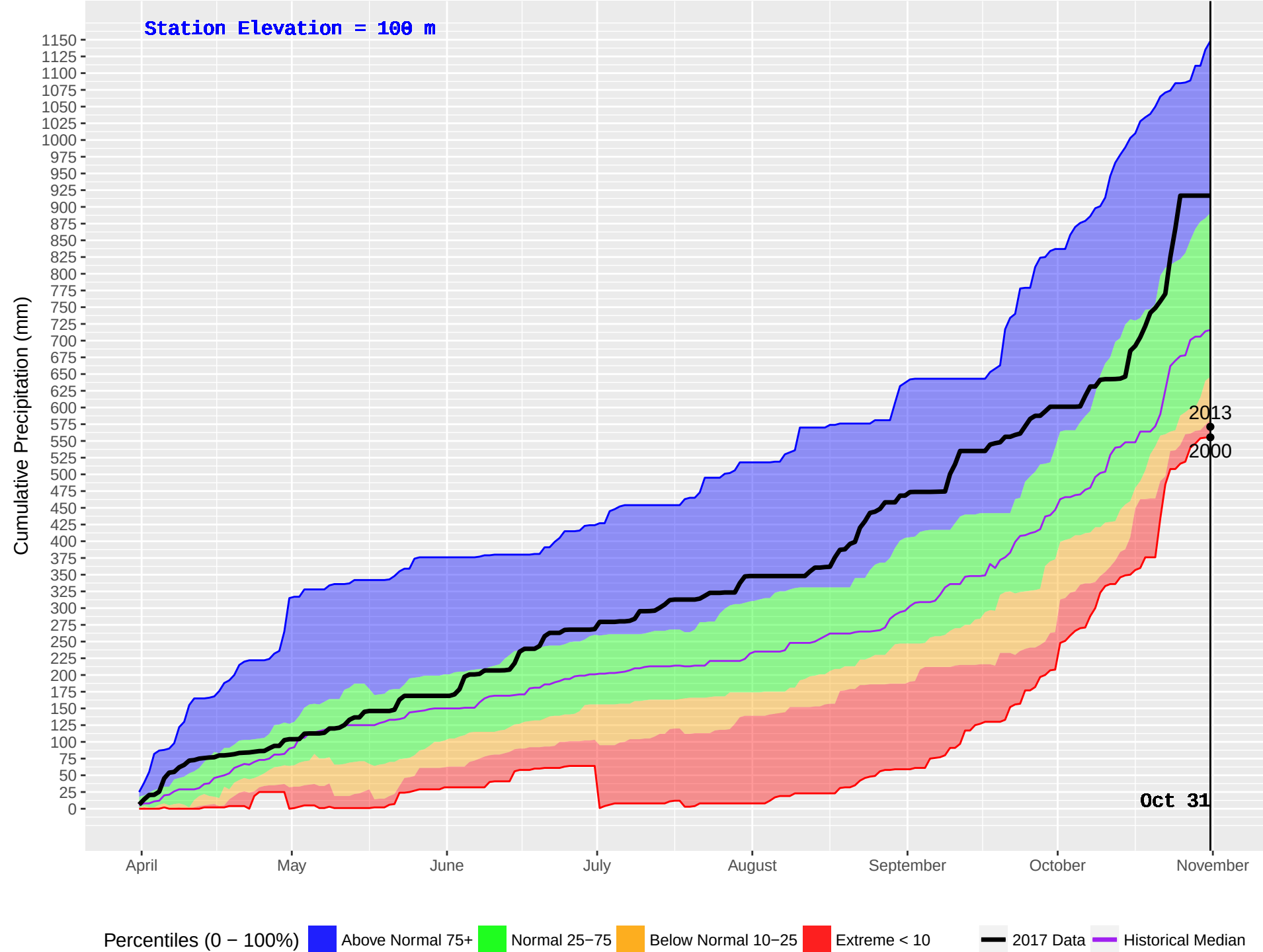
HONNA (93) : Historical (1986–2016) and Current (2017) Noon Cumulative Precipitation
