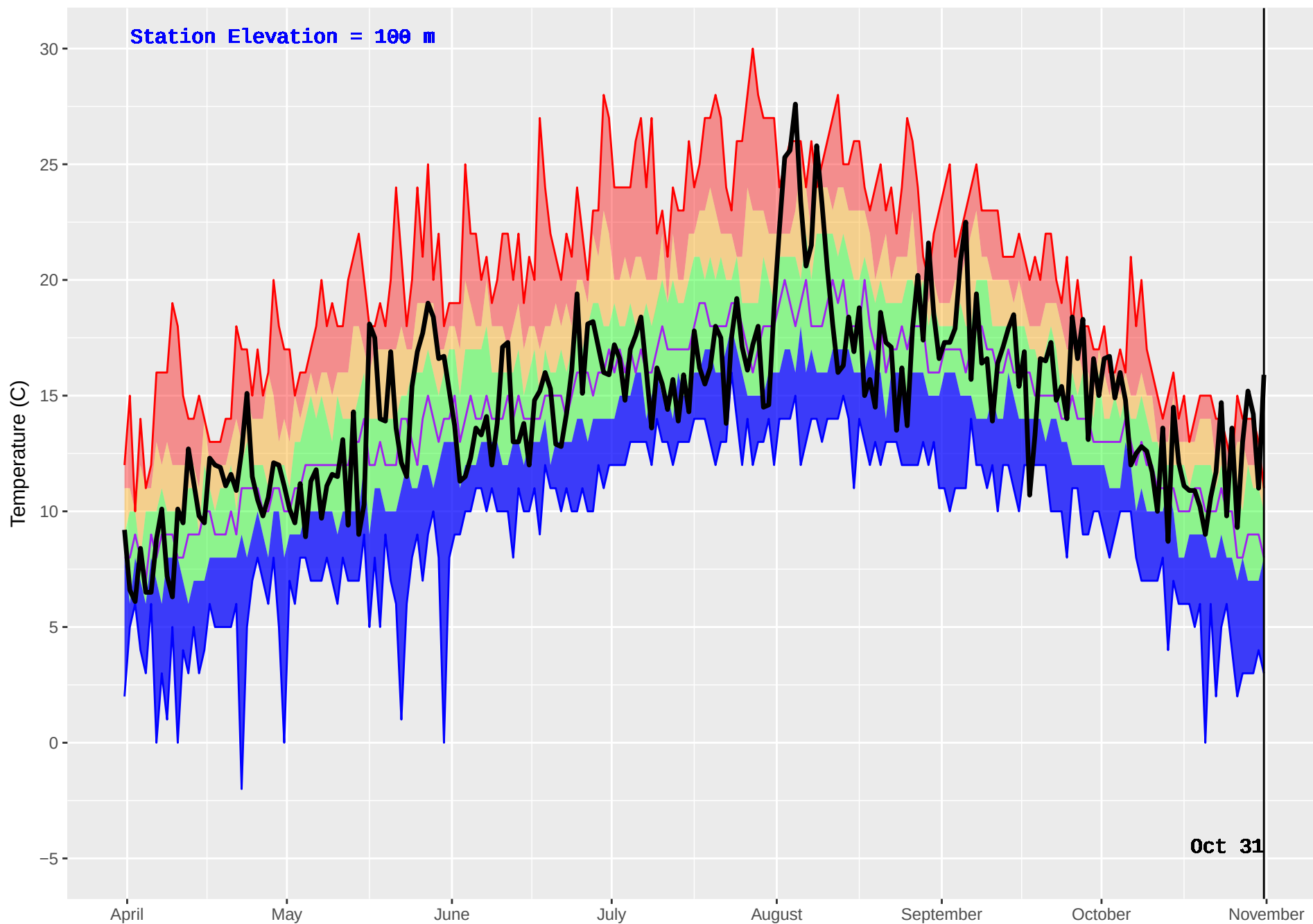
HONNA (93) : Historical (1986–2016) and Current (2017) Noon Temperature
